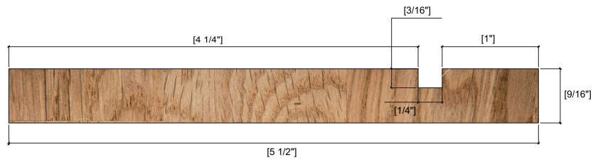
PFJ S4S 1 X 4 REVERSIBLE (11/16")
