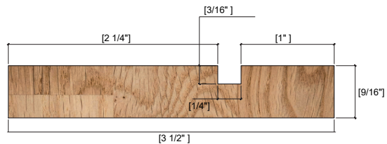
PFJ S4S 1 X 4 REVERSIBLE (9/16")
